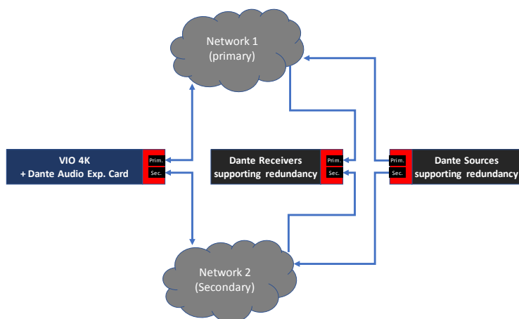
Diagram of VIO 4K equipped with Dante® audio option (Redundant configuration)
